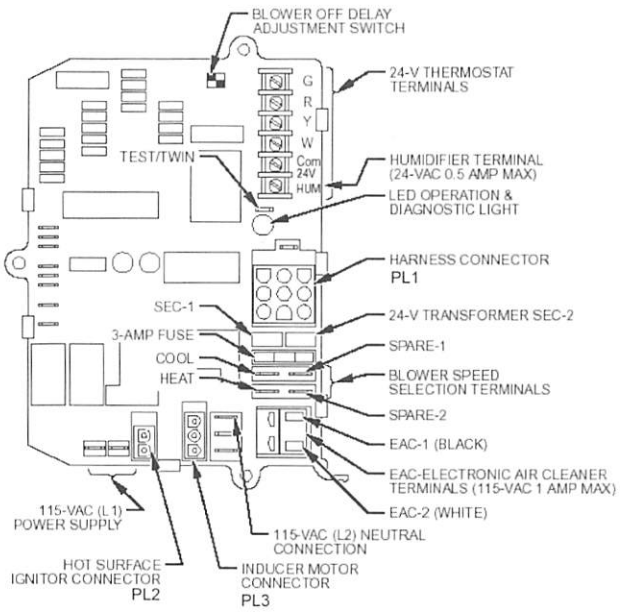
Figure 1 – Old Style Furnace Control Board
